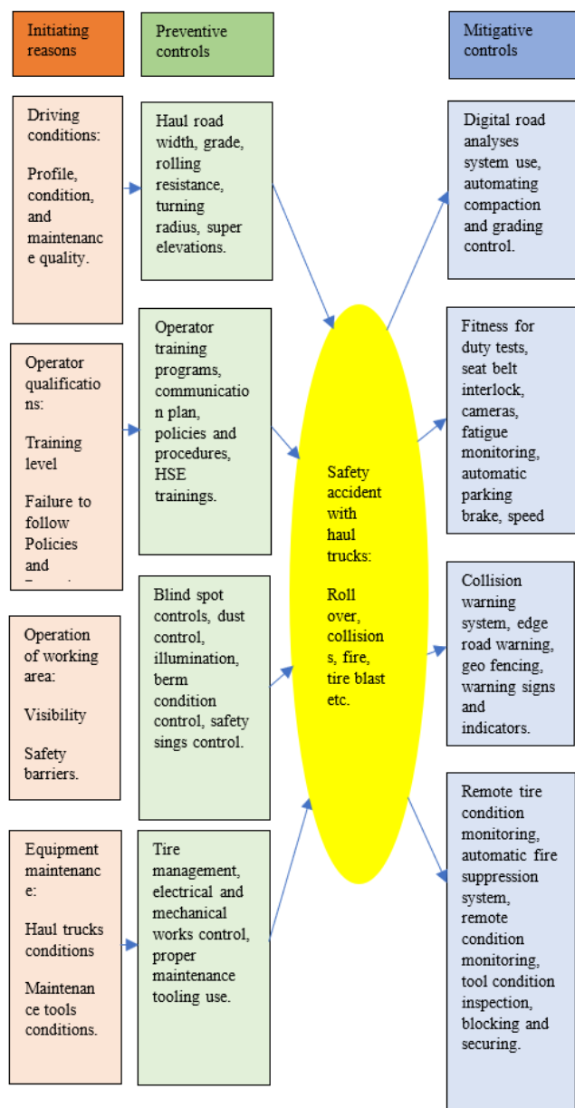
Figure 4. Bowtie diagram of mining haul truck operation failures analyzes of mines in Kazakhstan
